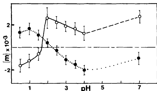
Fig. 3. Change of molar rotation of rG with pH. — 235 mμ, ..... 260 mμ.
